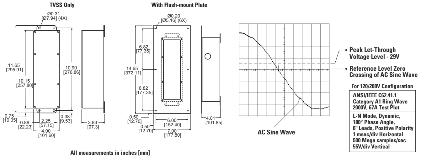
ANSI/IEEE C62.41.1-2002, C62.41.2-2002, & C62.45-2002 Measured Limited Voltage
